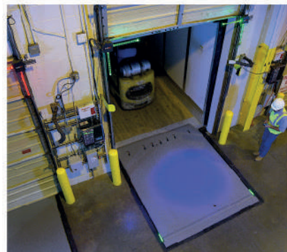
DOCK LEVELER
